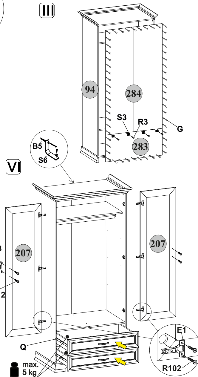
Шкаф 2DG2S Cupboard 2DG2S Szafa 2DG2S
