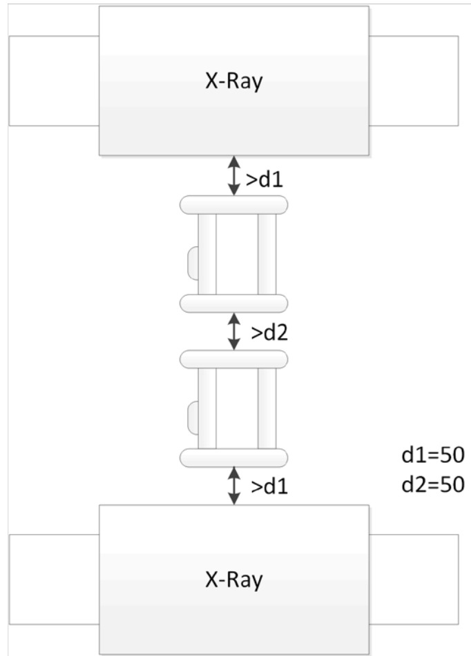
Figure 3-7 Multiple walk-through detectors site installation
