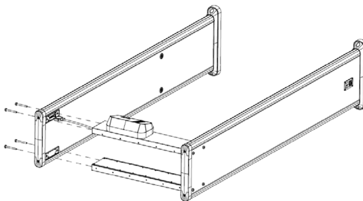
Figure 3-5 Fix beams (2)
