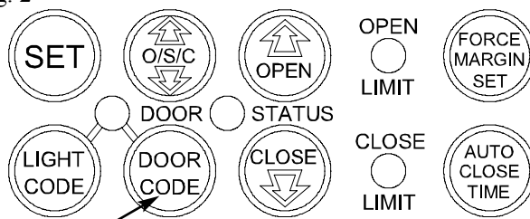
GDO-2 & GDO-4 Garage Door Opener Control Panel
