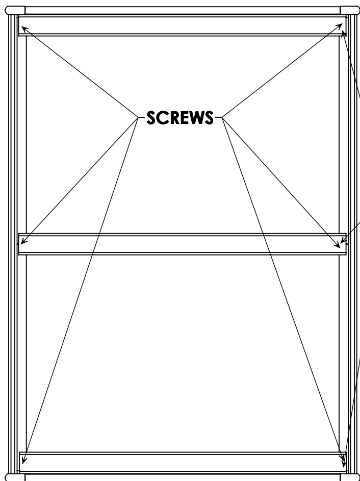
SLAT LOCATION FOR SUPPORT OF A FOUNDATION
