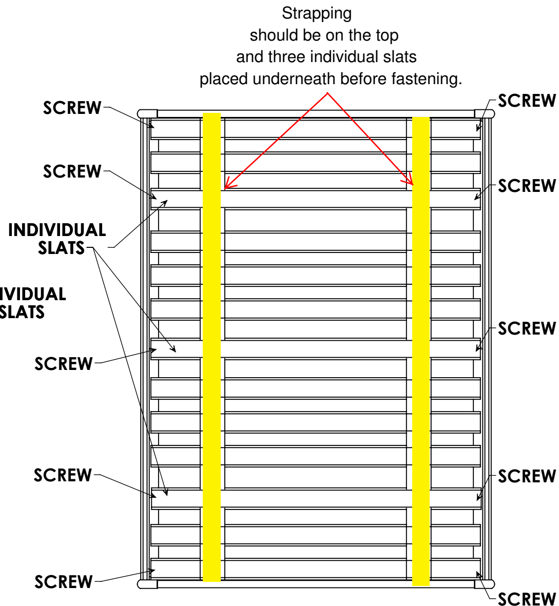
SLAT LOCATION WITH PURCHASED SLAT KIT
