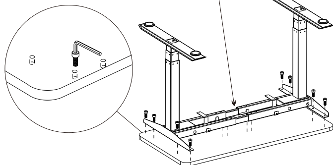
Predrilled
