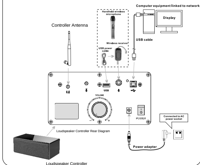
Connection and Installation Diagram of Equipment
