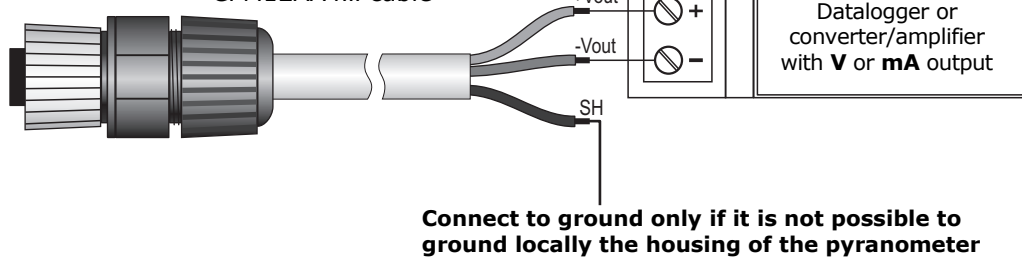
Fig. 4.1: LPPYRA-Lite connections
