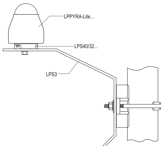
Fig. 3.4: fixing on LPS3 bracket
