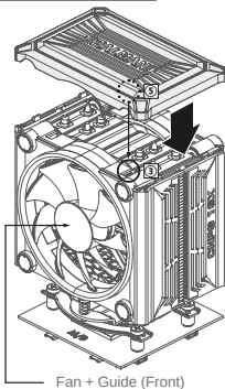
Top LED Cover
