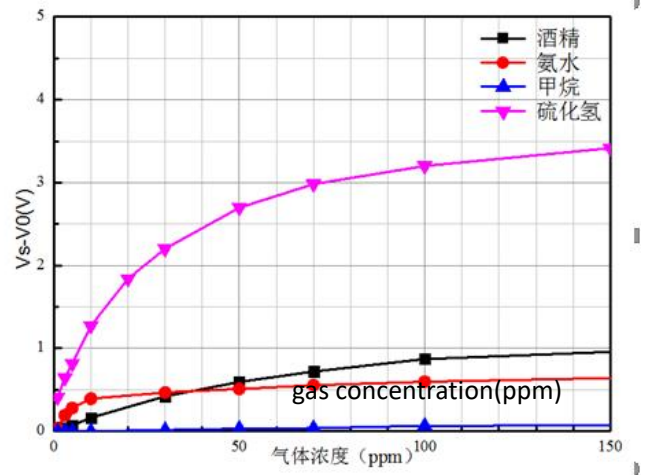
Fig6. Linearity character
