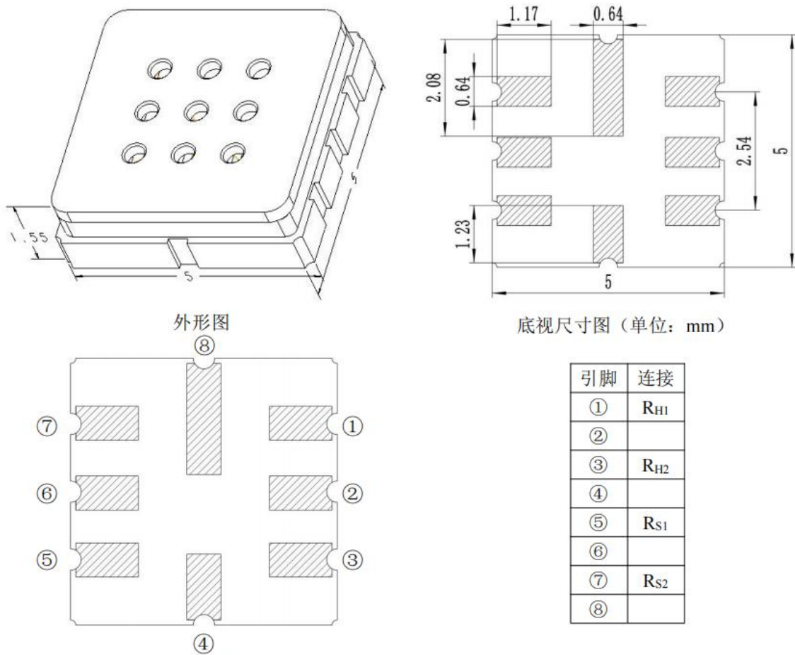
Fig1.Sensor structure
