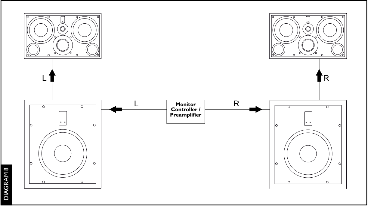
Diagram 8 – Typical Configuration – Stereo playback (Stereo Subs). A monitor controller or preamplifier output is connected to a single Input on each subwoofer. The corresponding Output of each subwoofer is connected to the Input of the main monitor on that channel. In this configuration, the Gain switch is normally set to 0dB. Note that it is also possible to connect the monitor controller output to both Left and Right channel Inputs on the subwoofer using a Y-Splitter cable. If connected in this way the "spare" output can be used to connect further subwoofers.
