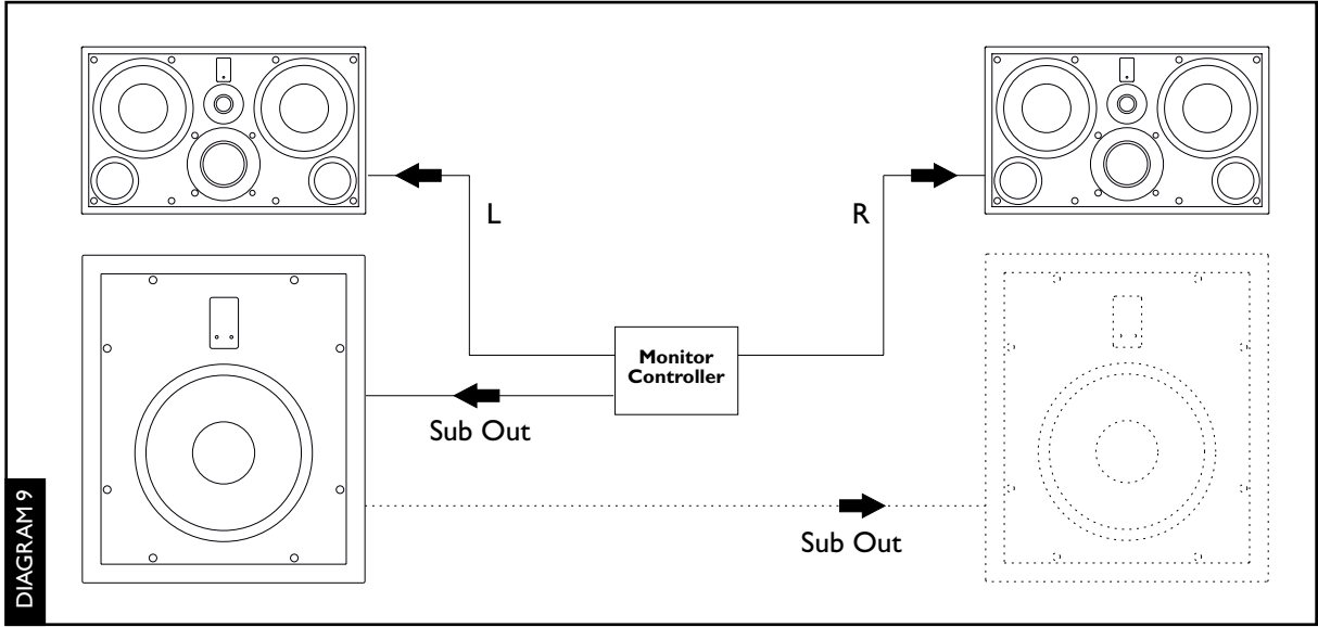
Diagram 9 – 2.1 Configuration – The subwoofer is driven by a monitor controller with a dedicated subwoofer output. Additional subwoofers may be daisy chained where more than one is required.
