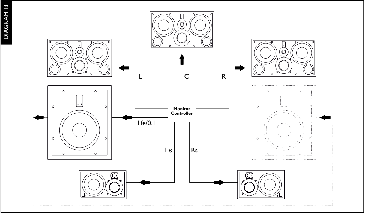
Diagram I3 – Typical Multichannel System wiring. Depending on the Monitor Controller output level and number of subwoofers, the Gain switches may need to be set to 6dB. Further subwoofers can be added to the system using the same “Daisy Chain” method shown. The system shown is an example and other configurations are available.
