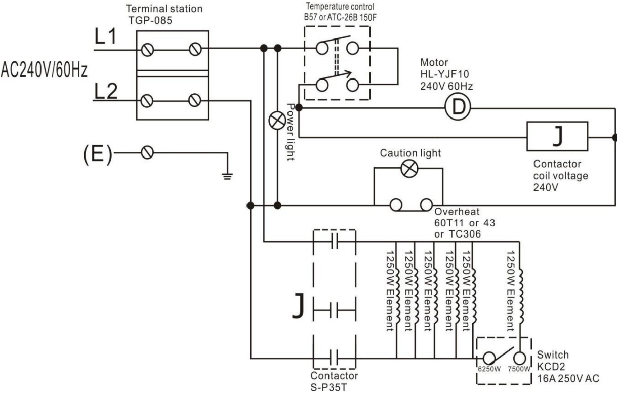
Circuit diagram Figure 7
