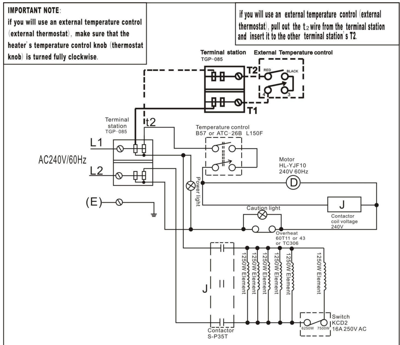
Circuit diagram Figure 10
