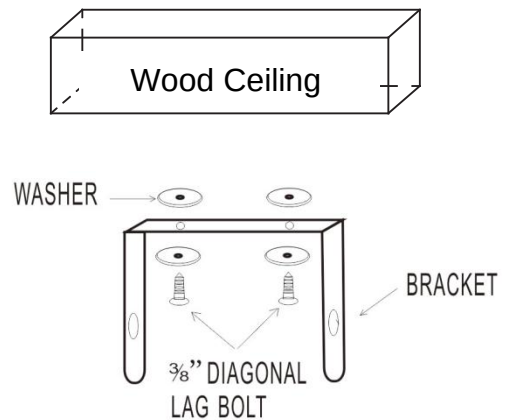
Figure 3b-Double-Screw Mounting
