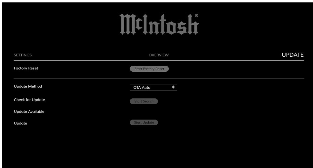
Figure 9– UPDATE submenu
