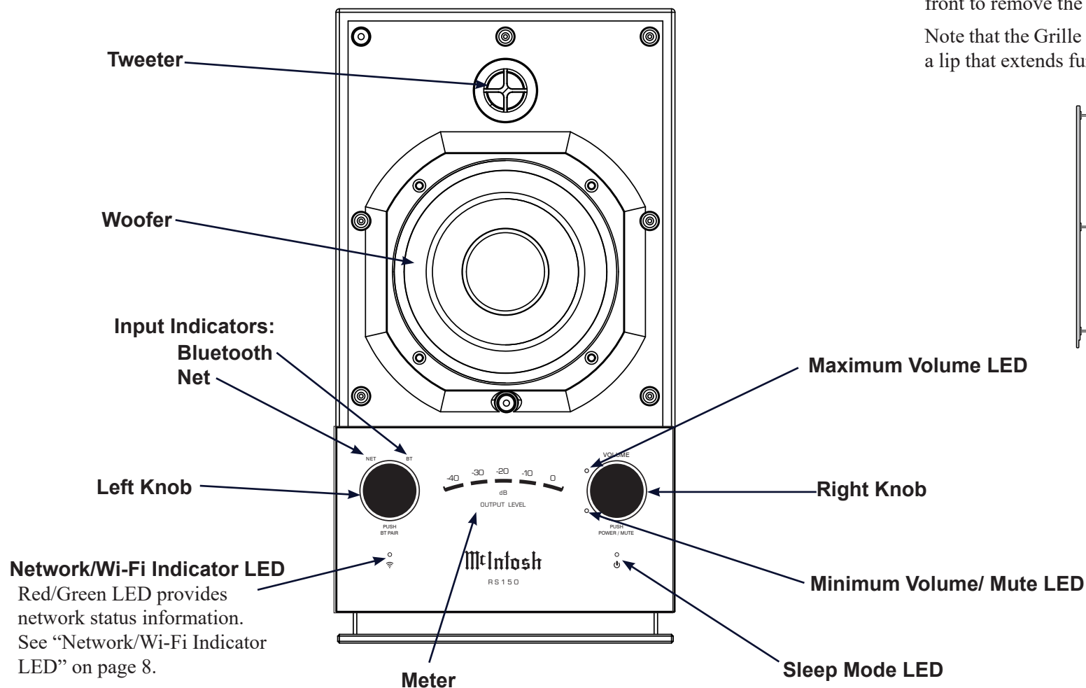
Figure 4– Front View
