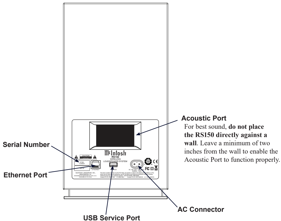
Figure 6— Rear View
