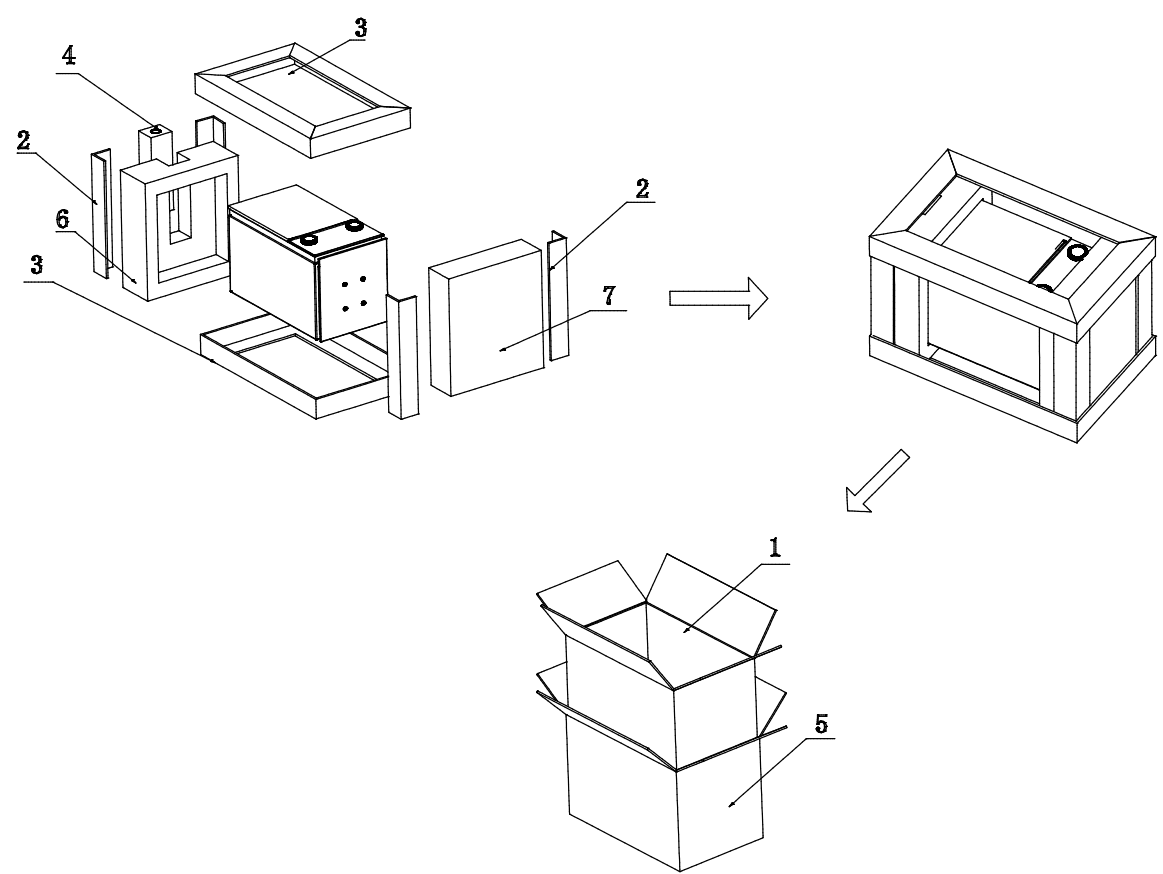
Figure 10– Packing Material
