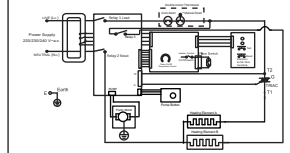
WIRING DIAGRAM -WITH ELCB, DC PUMP DPDT MODEL (FOR VIETNAM MODELS ONLY)
