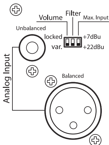
Rear connectors & DIP switches
