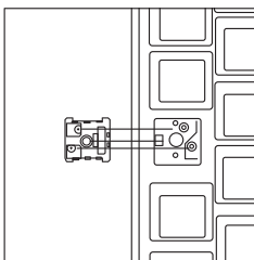
3.Align the new keyswitch's pins and base with the sockets and opening.
