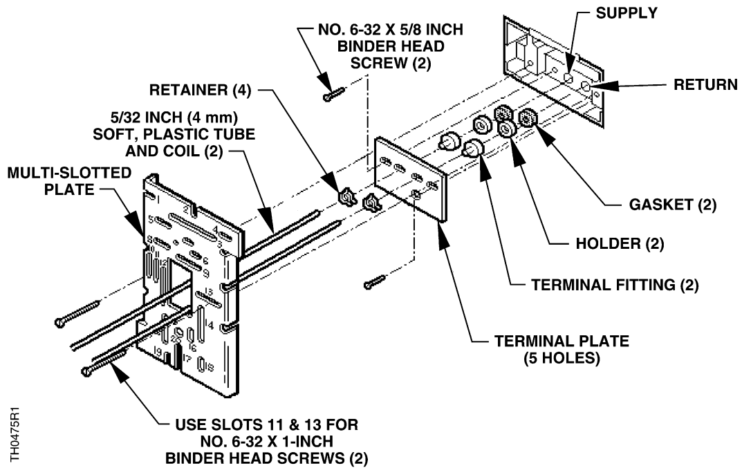
Figure 2. H & T 4000, 5000 Flush Box.
