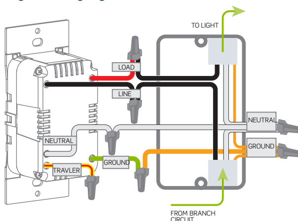
Single Pole Wiring Diagram
