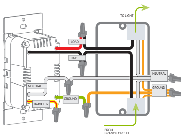
Single Pole Wiring Diagram
