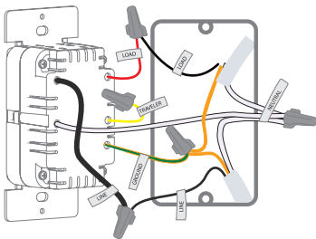
Single Pole Wiring Diagram
