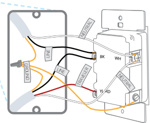
DD00R-DL OR DD0SR-DL COMPANION DEVICES
