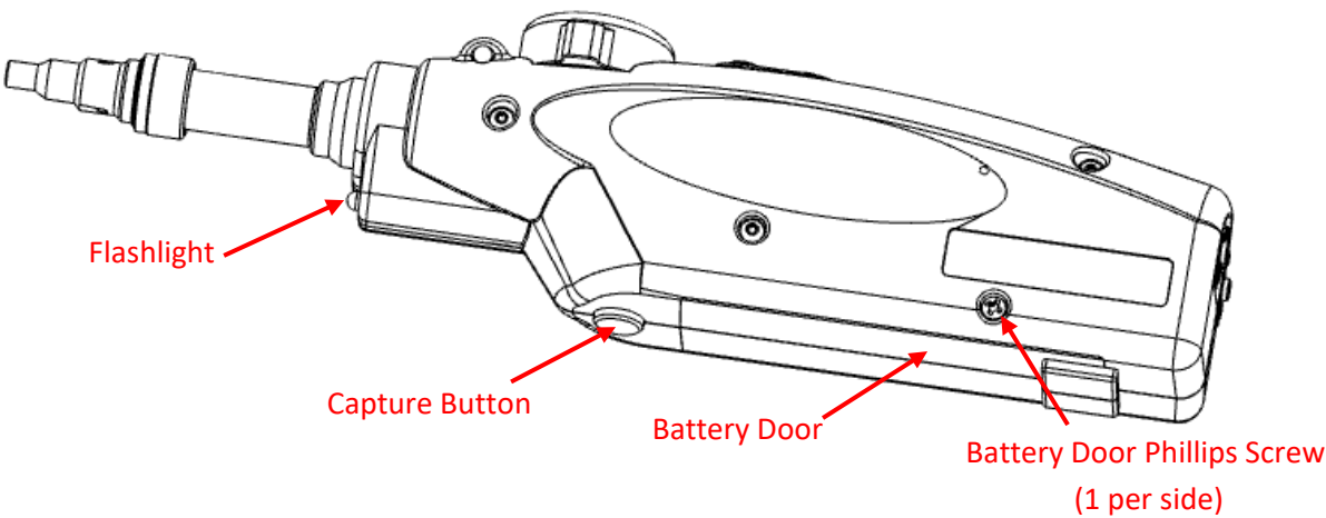
Figure 2 – Bottom View
