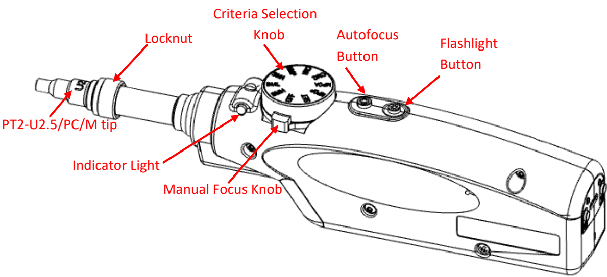
Figure 1 – Top View
