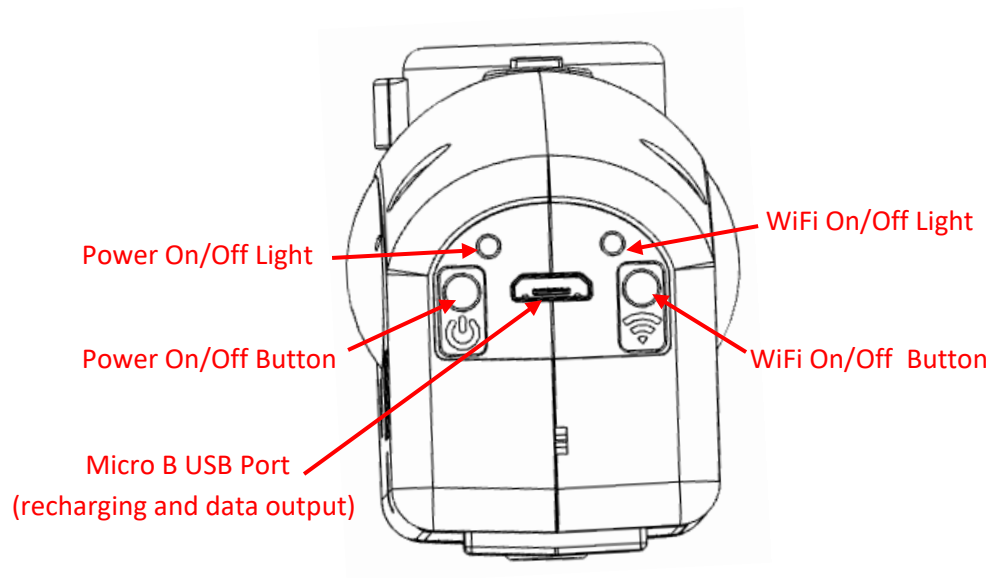
Figure 3 – Rear View
