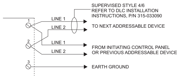
Figure 2 Wiring Information
