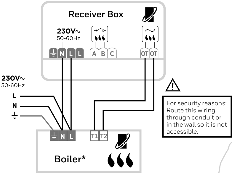
C) OpenTherm boiler
