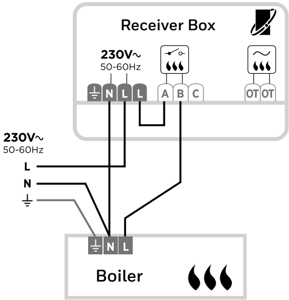
A) Basic 230V boiler
