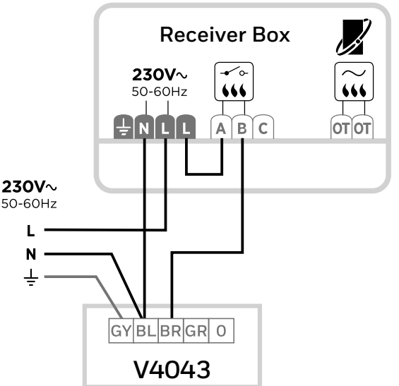
D) Two-port zone valve or S-plan
