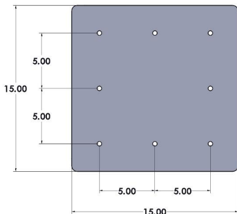
Bolt pattern for the Wide Base Floor Mount
