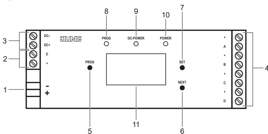
Fig. 1: Device components
