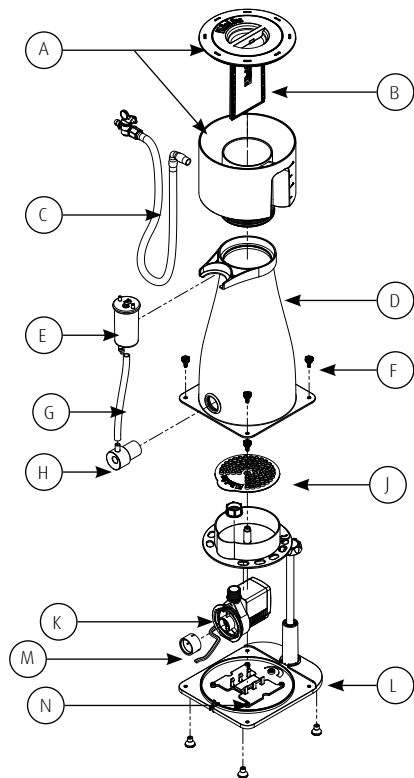
REEFER™ Skimmer Parts Diagram
