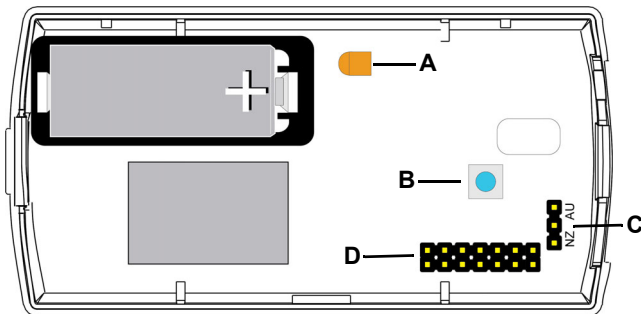
Figure 1 Integrated temperature/humidity transmitter internal components
