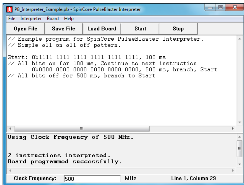
Figure 3: Graphical Interface of PulseBlaster Interpreter. The example shown creates a pulse that toggles all TTL bits on for 100 ms, then off for 500 ms, and repeats.
