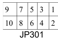
Figure 11: HW_Trig/Reset Header Pin-Out (SP57). Top-down view.
