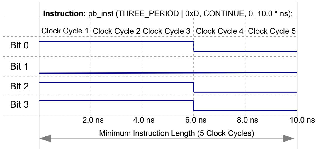
Figure 16: Example of the Short Pulse Feature. This example uses a 3 period duration. This example displays the output of 4 bits, but all bits are affected by the Short Pulse feature. Timing is done using a 500.0 MHz Clock.
