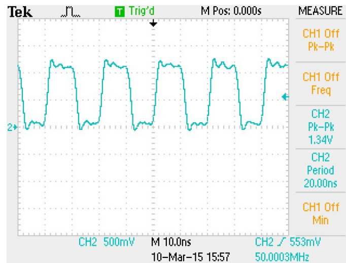
Figure 15: Example clock signal. Note that a small degree of voltage ripple is acceptable, so long as the voltage always remains above threshold for logical-high signals and below for logical-low signals.
