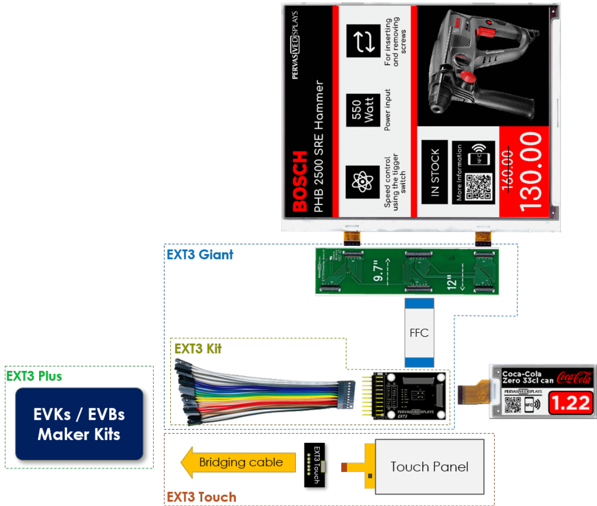
Figure 2 EXT3 Connectivity
