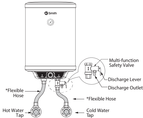
Figure 12 Installation Diagram
