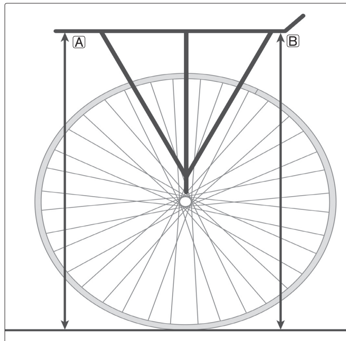
FIGURE A: The difference between heights A & B must be less than 3/4" (19.05 mm)
