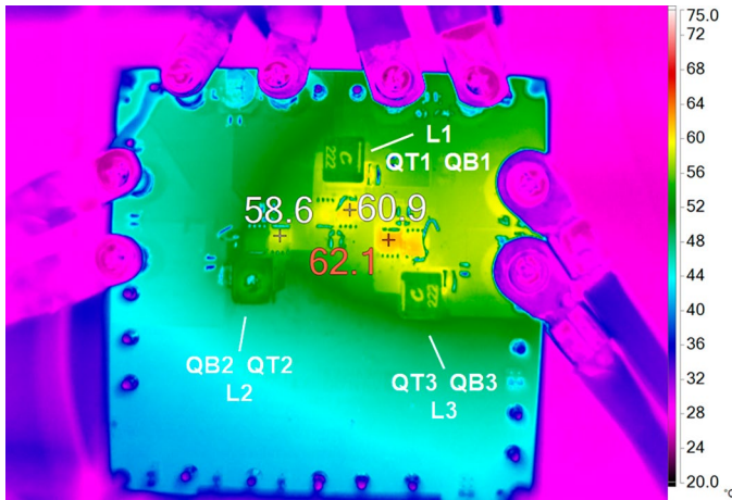
Figure 9. Thermal Image with Full Load on Each Rail at 12V IN , f SW = 380kHz, No Airflow, T A = 23°C, Markers Show the Hot Spot for Each Channel
