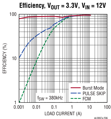
Figure 6. Efficiency of the 3.3V/12A Rail ( V_{OUT1} ) at 12V_{IN} for the Three Light Load Operating Modes, the Other Two Rails Were Disabled, No Voltage Was Applied to the EXTV_{CC} Pin and the PGOOD Pull-Ups Were Removed
