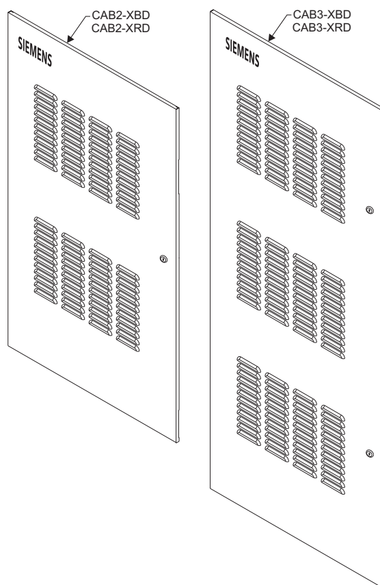
Figure 1 CAB2-XBD/-XRD And CAB3-XBD/-XRD Transponder Doors
