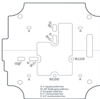
Figure 1. Mounting Template
