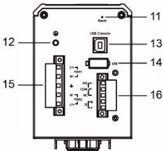
Bottom Panel View
