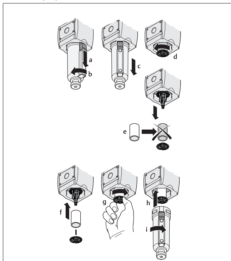
Fig. 6: Exchanging the filter |
