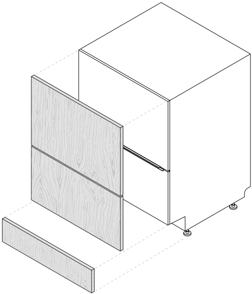
ISOMETRIC
