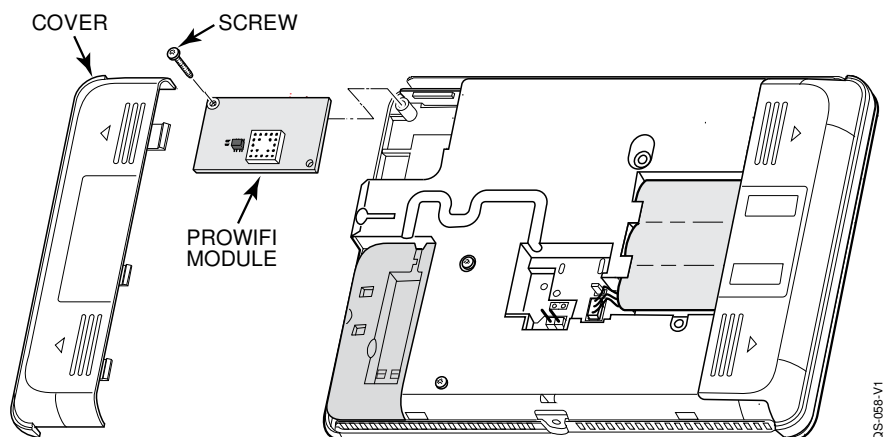
Figure 2. Installing the PROWIFI Module
