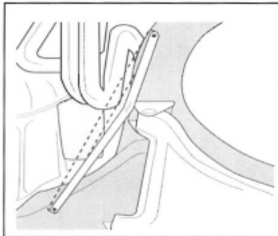
Illustration I (72-74 Frame Stiffeners)
