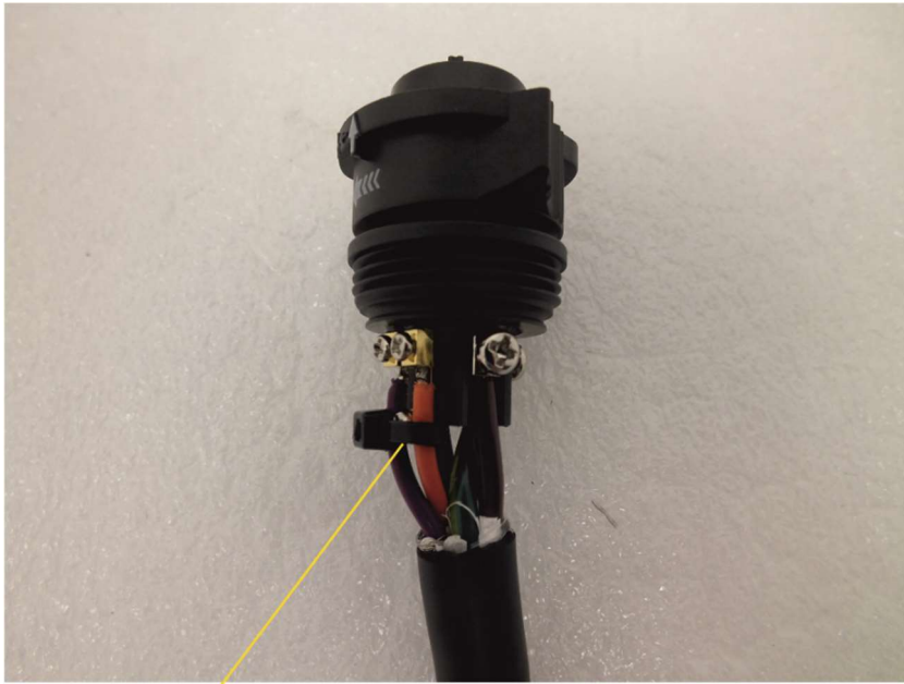
6 Cable binder
