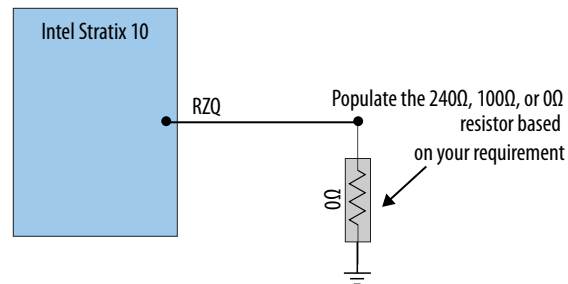
Figure 7. RZQ Pin for Banks 3[A, B, C, D]
