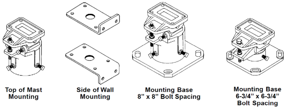
Figure 1-2 Mounting Bracket Options
