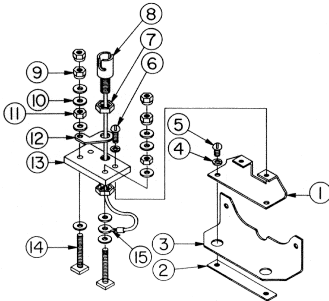
Figure 3-2 Lamp Support Bracket Replacement Parts Location
