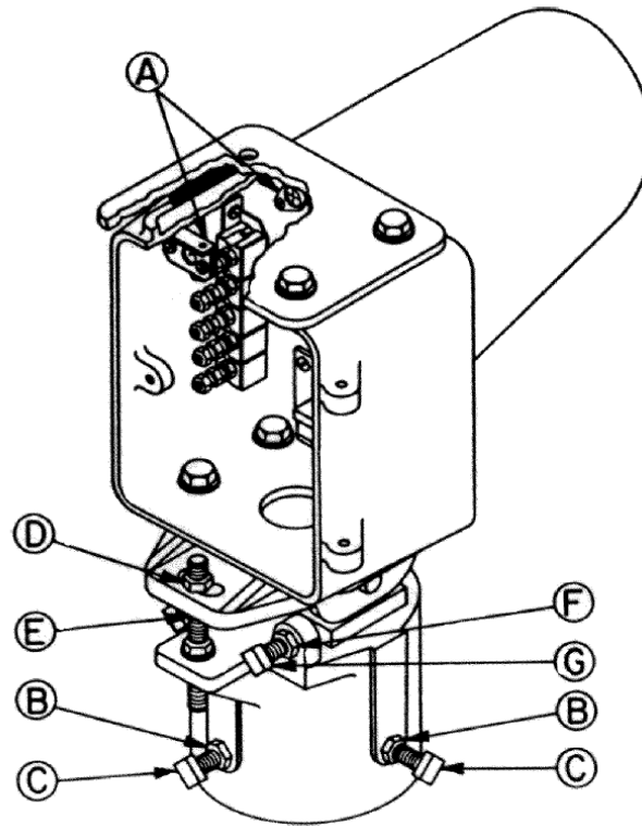
Figure 2-1 Lamp Alignment
