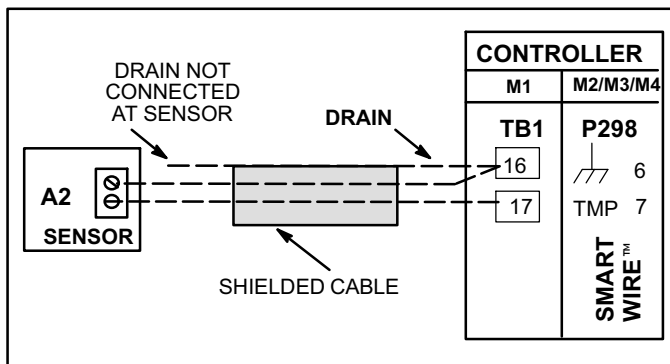
Figure 1. Sensor Wiring
