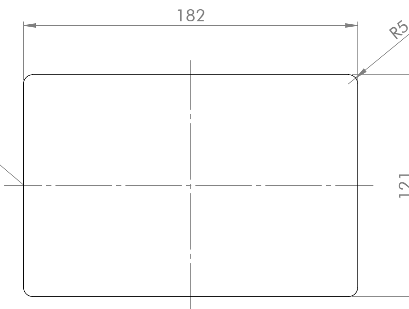
cut-out counterplate
