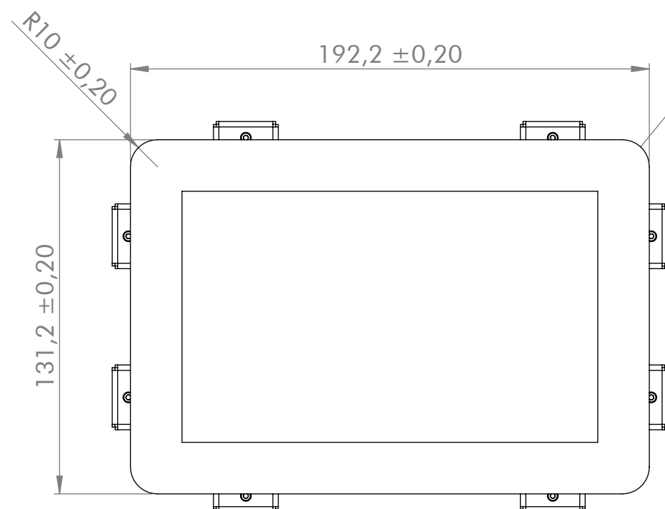
cut-out front- & spacerplate*
