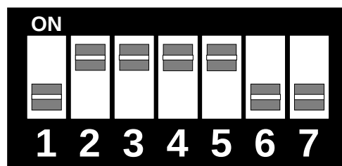
Figure 1 - RS-232 Mode
