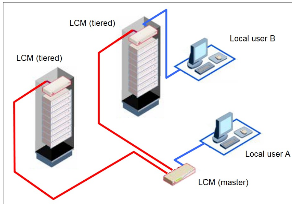
Figure 5. Tiered consoles
