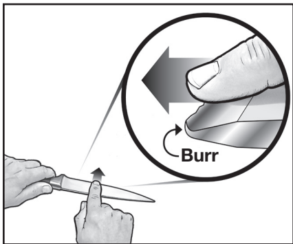
Figure 2. Develop a distinct burr along knife edge before honing in Stage 2. Burr can be detected by sliding finger across and away from the edge. Caution! See text.
