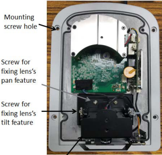
Calibration for tuning lens's vertical (-5 to 10° )and horizontal (+/- 5° ) position
