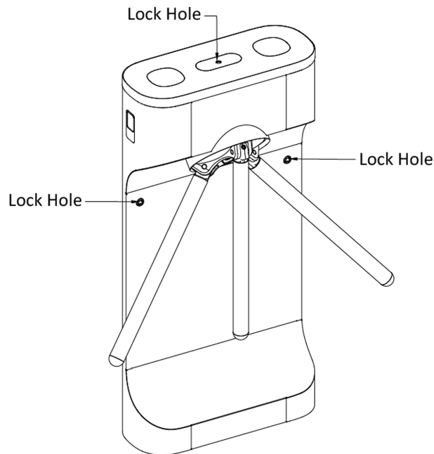
Figure 3-1 Lock Holes
