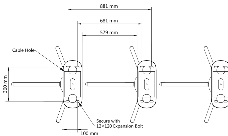
Figure 3-3 Installation Footprint
