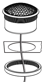
Option 1: Flush mounting
