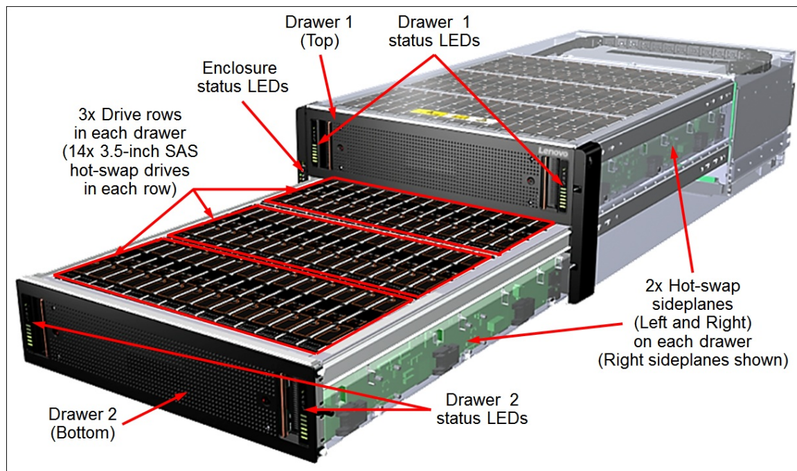
Figure 5. Front view of the D3284 drive enclosure
