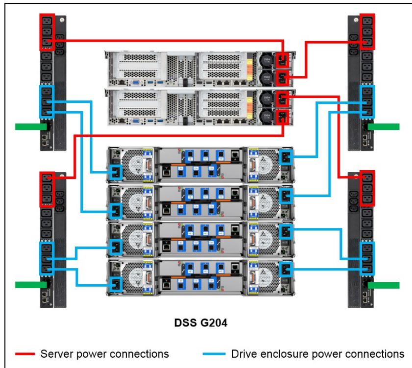
Figure 9. Power distribution topology
