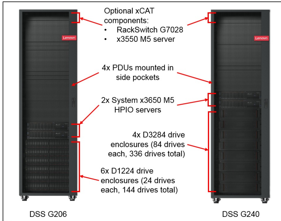
Figure 7. DSS-G components
