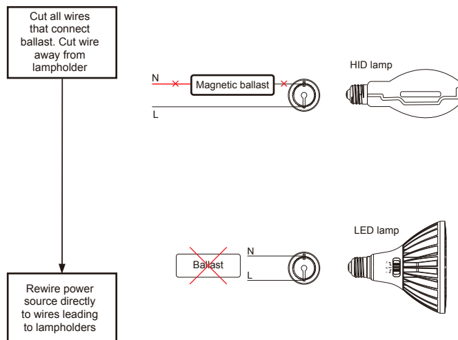
Diagram 5 – Magnetic ballast fixture wiring modification
