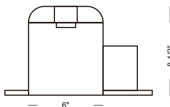
Diagram 2 – Minimum lamp compartment dimensions (for enclosed fixtures)
