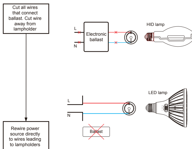
Diagram 4 – Electronic ballast fixture wiring modification
